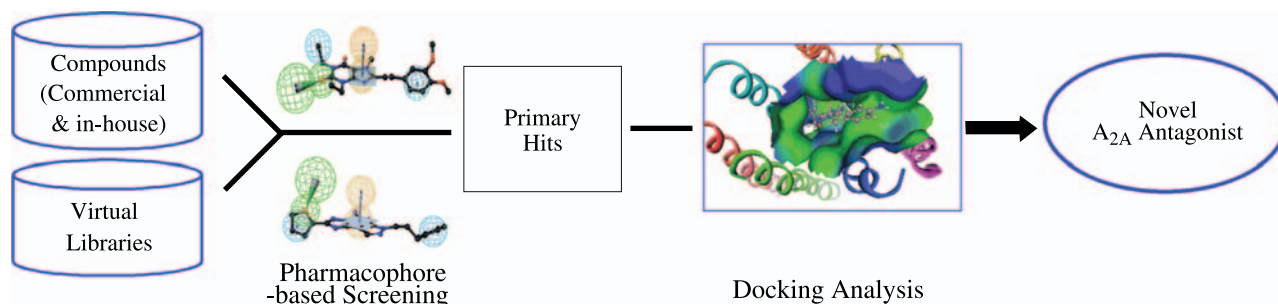
Fig. 6. Proposed virtual screening approach for novel A 2A antagonist
