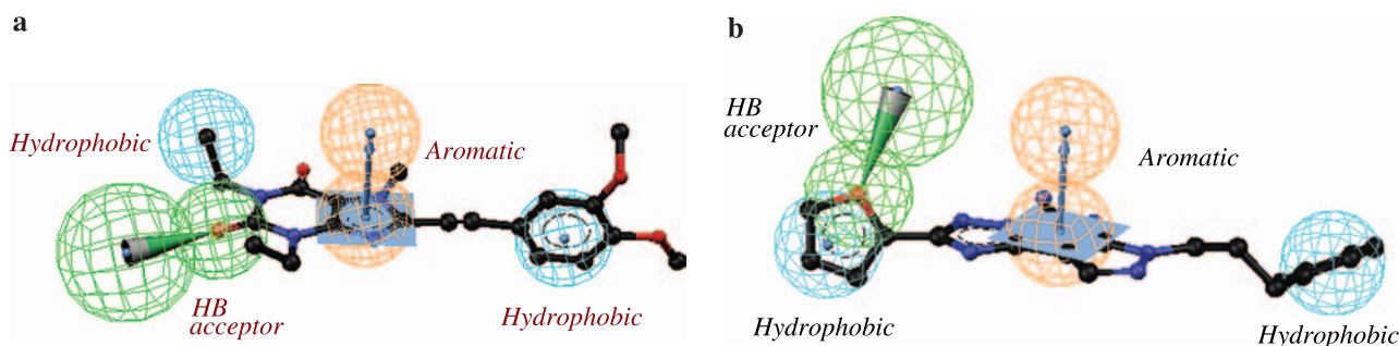
Fig. 5. Extracted pharmacophore models based on binding mode from docking analysis. (A) A representative of four featured pharmacophore model from xanthine type A 2A antagonist. (B) A representative of four featured pharmacophore model from non-xanthine type A 2A antagonist. Pharmacophore features are color-coded: green represents hydrogen bond acceptor; orange represents ring aromatic; light blue represents hydrophobic (for an interpretation of the reference to colour in this figure, the reader is referred to the online version of this paper under www.springerlink.com )
