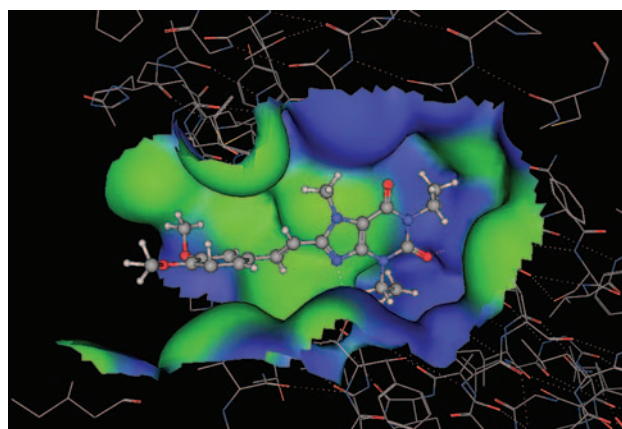
Fig. 2. Theoretical models of the A 2A binding site complexed with compound KW6002. The molecular surface is color-coded by hydrophobicity properties. The green is for hydrophobic, blue for hydrophilic. The constituents of the pocket are defined by those residues within a distance of 6 Å from the ligands. For a better illustration of the binding modes, residues at one side of the pocket are hidden (for an interpretation of the reference to colour in this figure, the reader is referred to the online version of this paper under www.springerlink.com )
