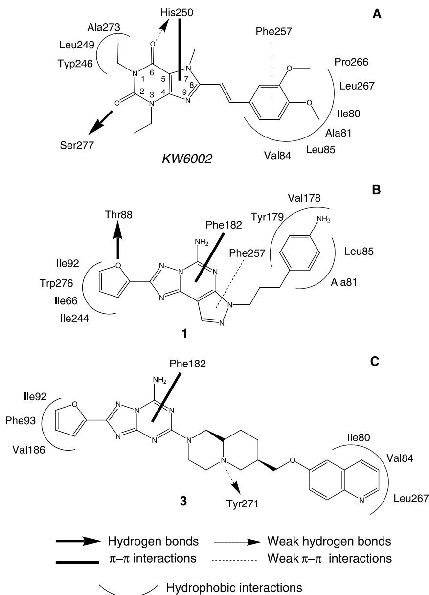
Fig. 3. Binding mode of the A 2A antagonists. (A) Binding mode of KW6002 , (B) Binding mode of compound 1 . (C) Binding mode of compound 3
