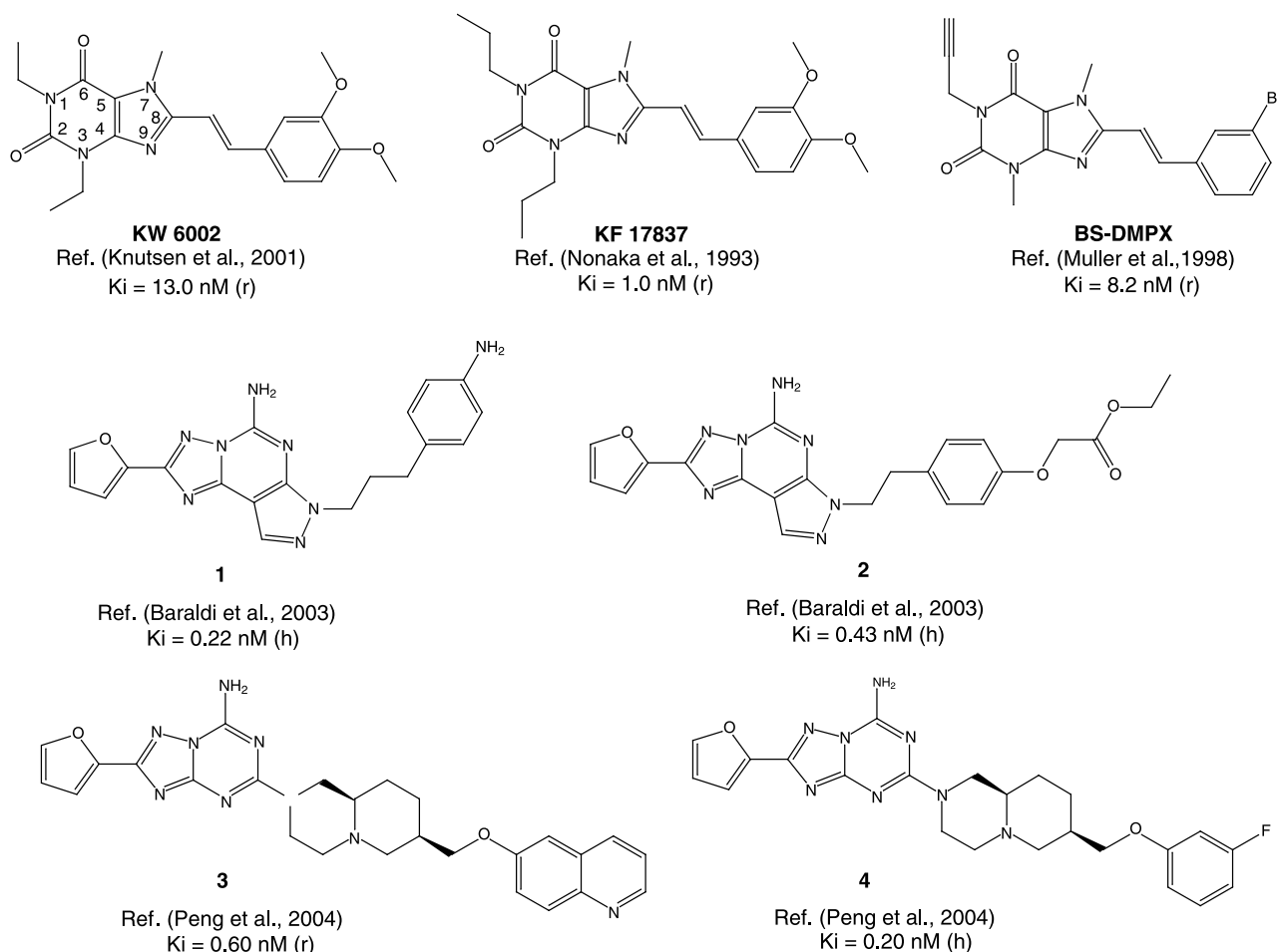
Fig. 1. Compounds selected for docking study and SAR analysis. (r rat; h human)
