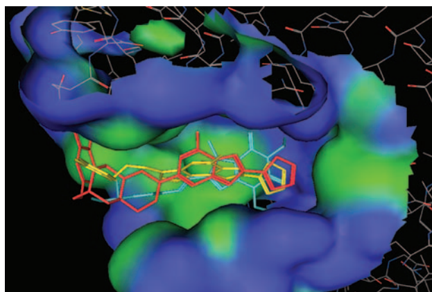
Fig. 4. Molecular surface of the active pocket of A 2A adenosine receptor. KW6002 (cyan), compound 1 (yellow) and compound 3 (red) are docked in the binding pocket. The molecular surface is color-coded by hydrophobicity properties. The green is for hydrophobic, blue for hydrophilic. The constituents of the pocket are defined by those residues within a distance of 6 Å from the ligands. For a better illustration of the binding modes, residues at one side of the pocket are hidden (for an interpretation of the reference to colour in this figure, the reader is referred to the online version of this paper under www.springerlink.com )
